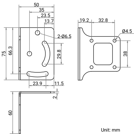
Installation Bracket:
