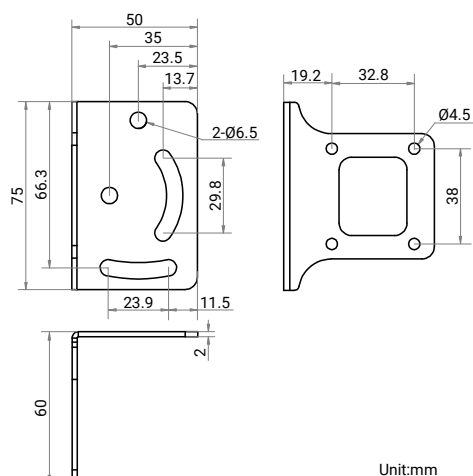
Installation Bracket:
