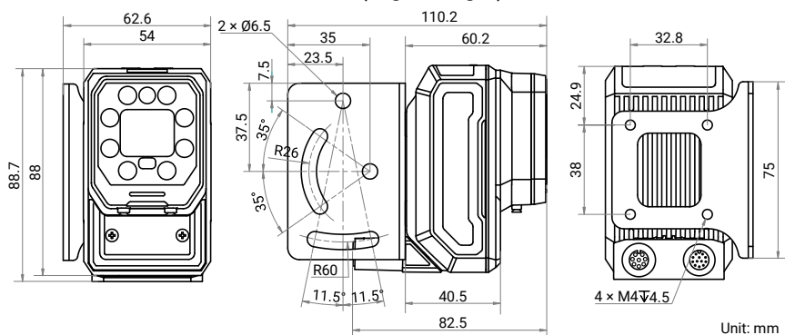
Installation Bracket:
