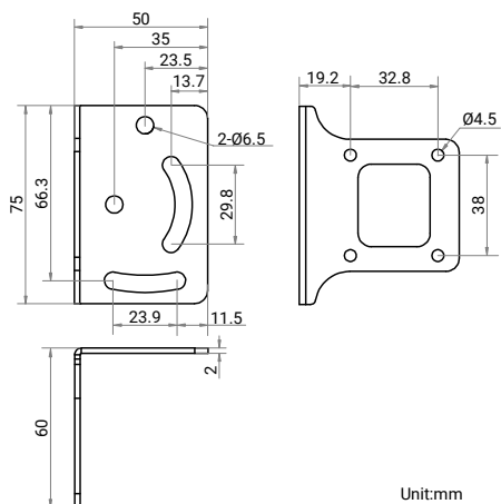
Installation Bracket:
