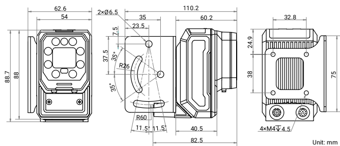
Installation Bracket:
