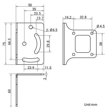
Installation Bracket:
