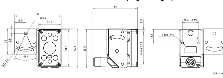
Device and Installation Bracket 1 (Right Angle)
