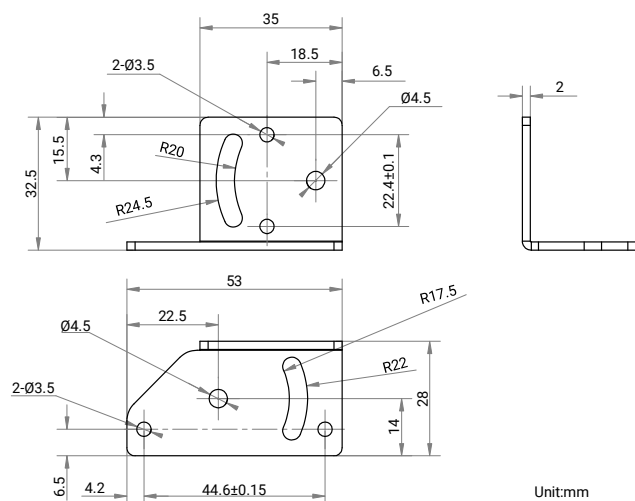
Bracket
