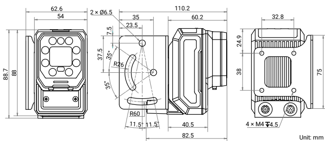
Installation Bracket:
