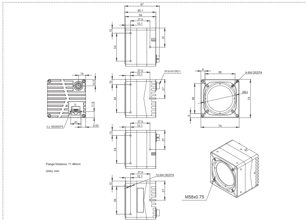
MARS-5000-24GTM/C M58-D1, M58-mount, flange distance:11.48mm
