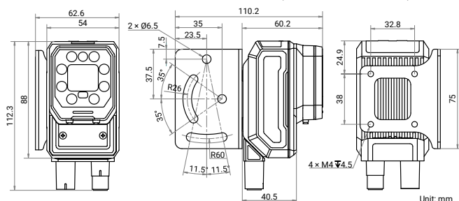
Device and Installation Bracket (Right Angle):
