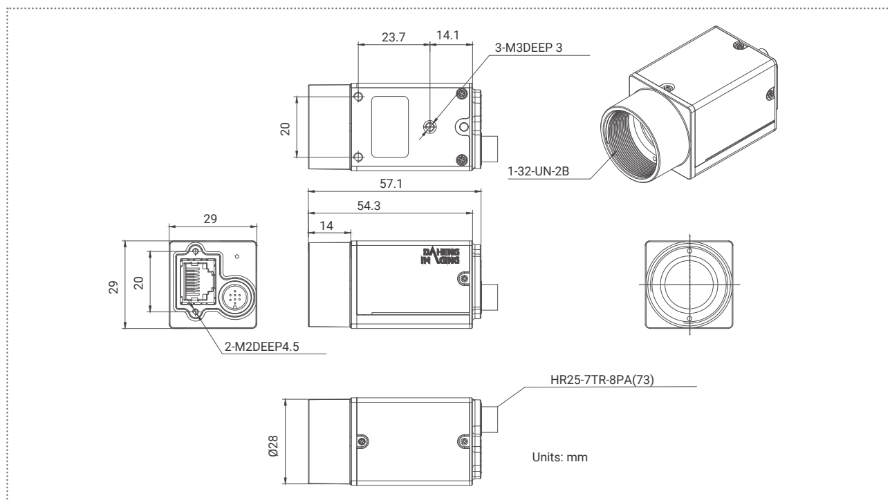
MER2-507-23GM/C-P
