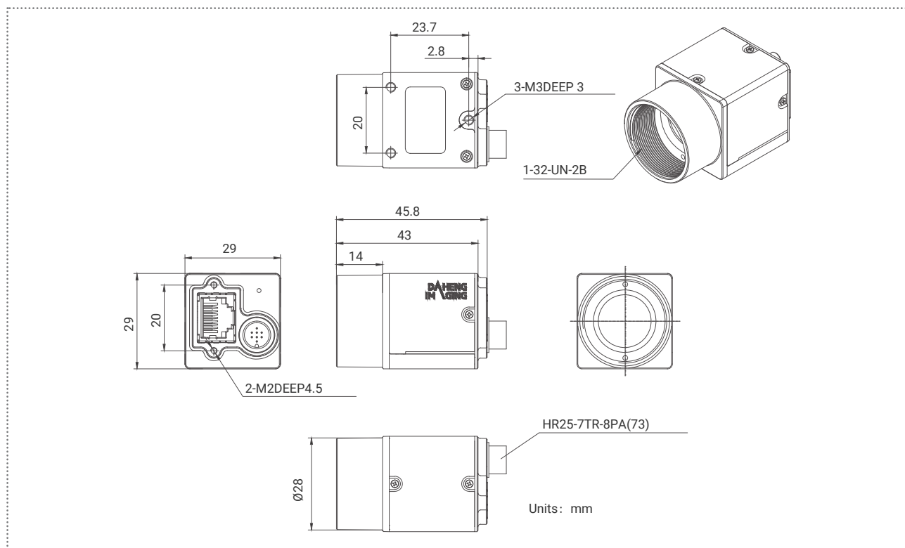
MER2-507-23GM/C
