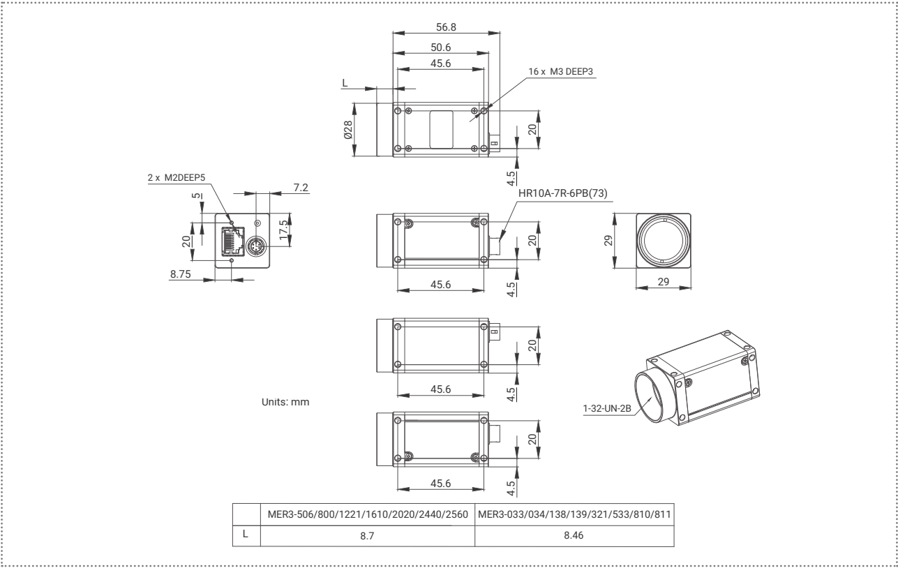
Without Heat Dissipation Fins
