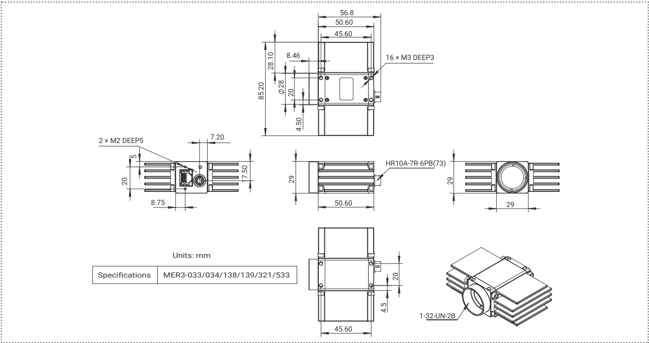
With Heat Dissipation Fins
