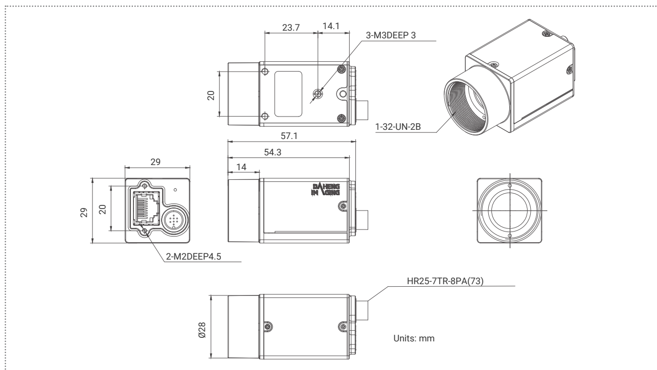
MER2-1220-9GM/C-P
