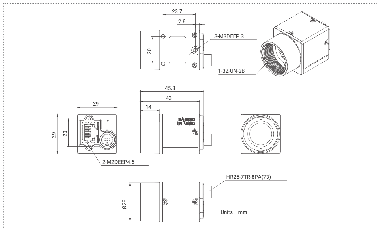
MER2-1220-9GM/C
